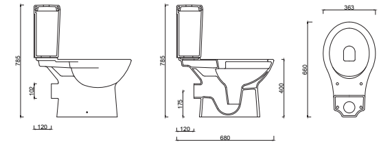
TR03KLZ00 TRIA RIMLESS DUVARA YARIM DAYALI KLOZET TR02RZV00 REZERVUAR TR04KLZ00 TRIA RIMLESS SEMI BACK TO WALL CLOSET TR02RZV00 CISTERN
