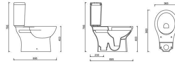
TR23KLZ00 TRIA RIMLESS DUVARA DAYALI KLOZET TR02RZV00 REZERVUAR TRO0KRK48 KLOZET + REZERVUAR TR24KLZ00 TRIA RIMLESS UNIVERSAL BACK TO WALL CLOSET TR02RZV00 CISTERN
