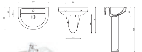
K004LVB01 COMPACT LAVABO (45x55) K001AYK00 KOLON AYAK CA02AYK00 YARIM AYAK K004LVB01 COMPACT WASHBASIN (45x55) K001AYK00 PEDESTAL CA02AYK00 SEMI PEDESTAL
