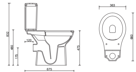
CA19KLZ00 CARMINA RIMLESS ENGELLİ KLOZET (ARKA ÇIKIŞLI) CA09RZV00 REZERVUAR CA20KLZ00 CARMINA RIMLESS DISABLED CLOSET (P-TRAP) CA20RZV00 CISTERN
