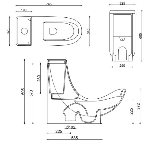
WH01KLZ029800 WC HEALTH DUVARA DAYALI KLOZET WH01KLZ029800 WC HEALTH UNIVERSAL BACK TO WALL CLOSET
