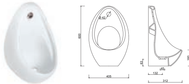
TP05PSR00 | TP05PSR00 ANKASTRE FOTOSELLİ PİSUVAR | BUILT - IN SIPHONIC URINAL
