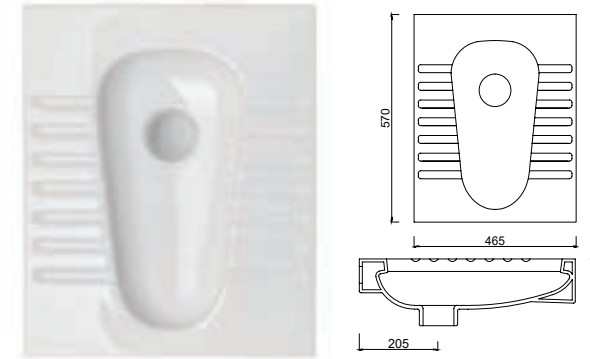
TP10HLT00 | TP10HLT00 ÇEVRE YIKAMALI HELA TAŞI (47X57) | SQUATTING PAN BOX RIM
