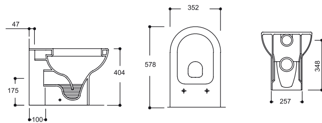
K003DTK00 COMPACT DUVARA DAYALI TEK KLOZET K004DTK00 COMPACT SINGLE BACK TO WALL CLOSET
