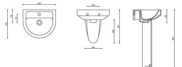
TP09LVB01 COMPACT BANTLI LAVABO (40x46) K001AYK00 KOLON AYAK K002AYK00 YARIM AYAK TP09LVB01 COMPACT WASHBASIN "D-SHAPED" (40x46) K001AYK00 PEDESTAL K002AYK00 SEMI PEDESTAL
