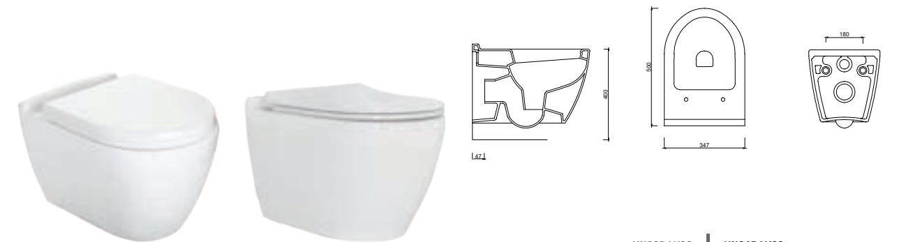
UN03DAK00 | UN04DAK00 UNO DUVARA ASMA KLOZET (GİZLİ MONTAJ) | UNO WALL HUNG CLOSET (HIDDEN FIXATION)
